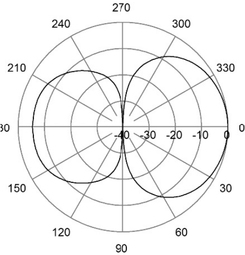
E-Plane | 459 MHz
